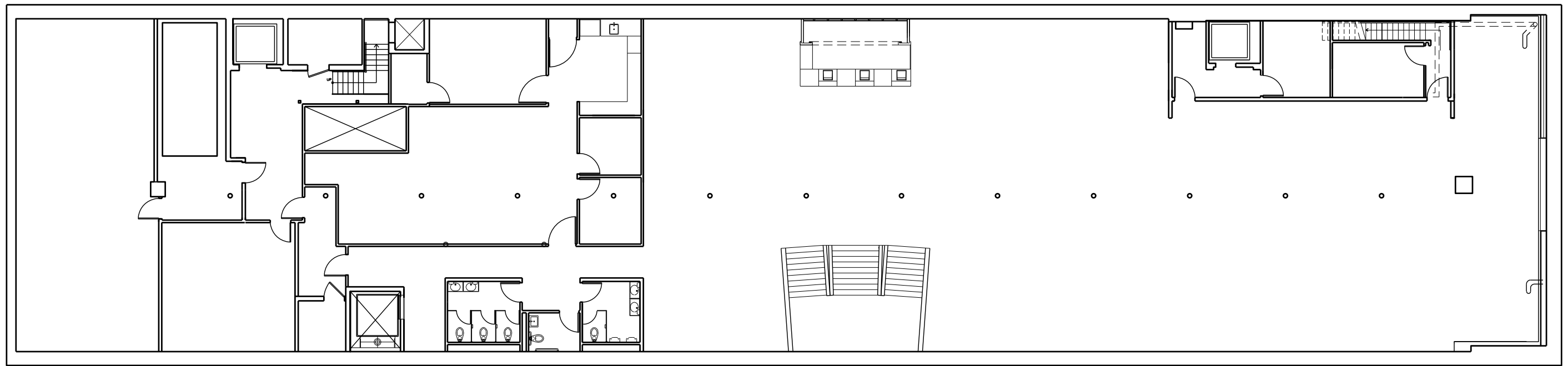
CELLAR PLAN SCALE: 1/16" = 1'-0"
